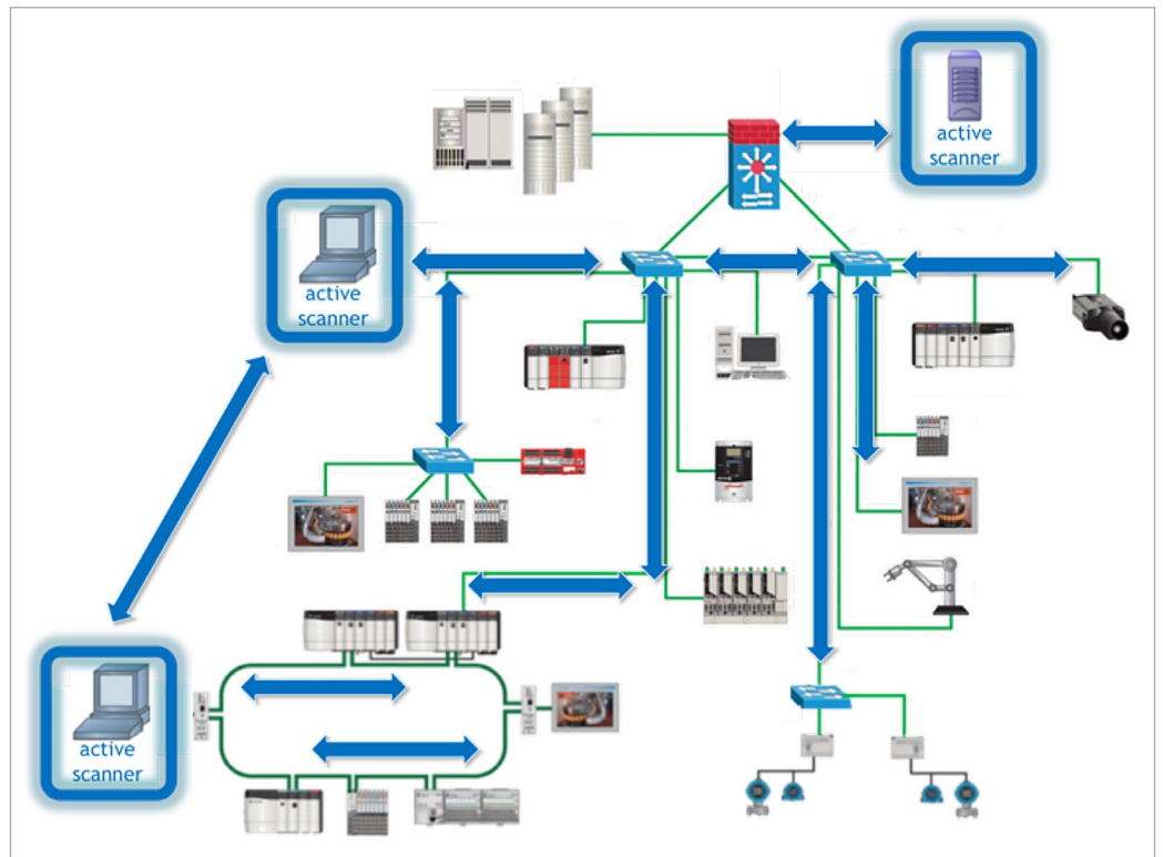
Figure 7. Network Architecture with Active Scanners
