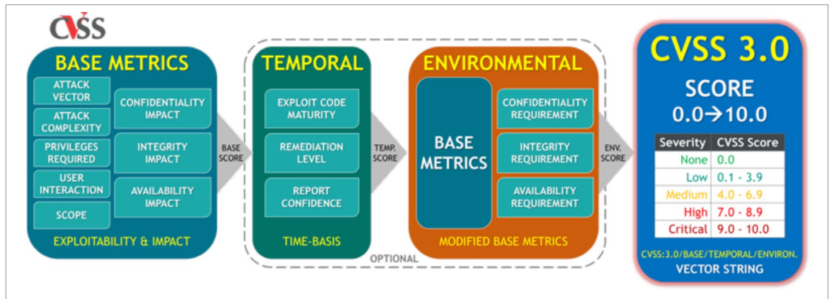
Figure 10. CVSS 3.0 Base Score Calculation
